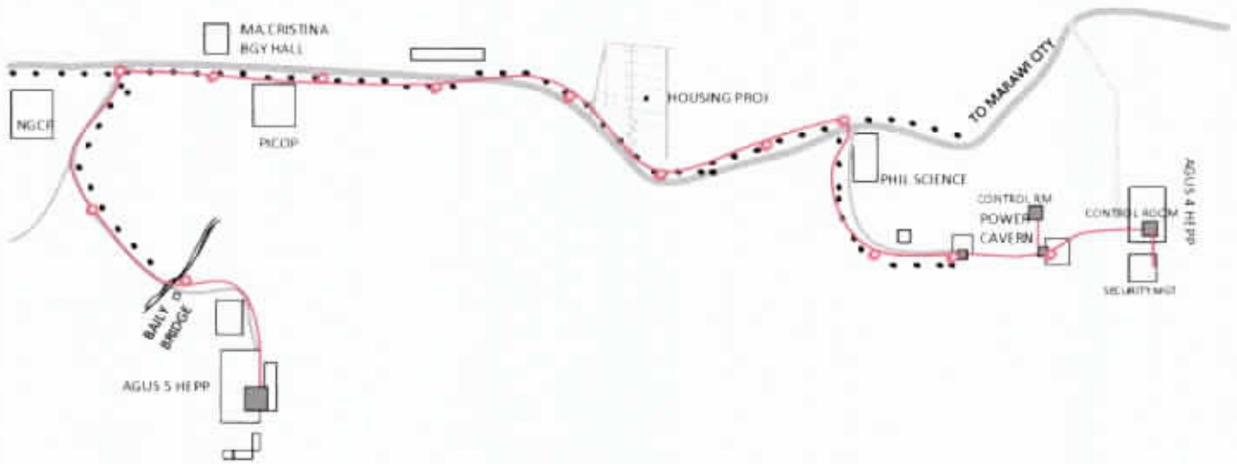
PROPOSED FIBER OPTIC TELECOMMUNICATION BACKBONE FOR DATA ,VOICE , INSTRUMENTATION, VIDEO ,AND SECURITY MANAGEMENT FOR AGUS 4 AND AGUS 5 HYDRO ELECTRIC PLANT COMPLEX
